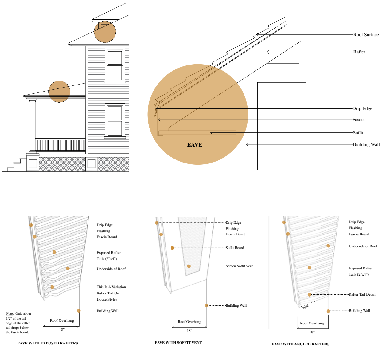
Figure 6.9: Eaves and Overhangs
