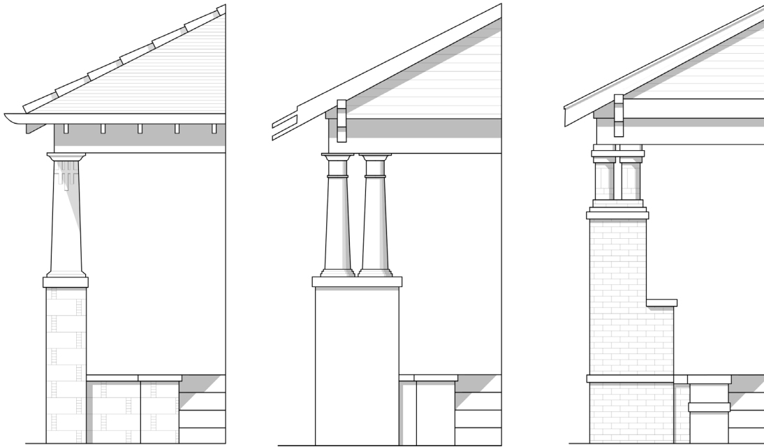
Figure 6.13: Bungalow and Craftsman Porch Column Variations
